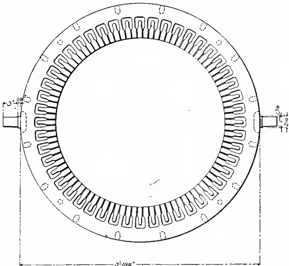
Fig. 5363. Plan of Chill.
